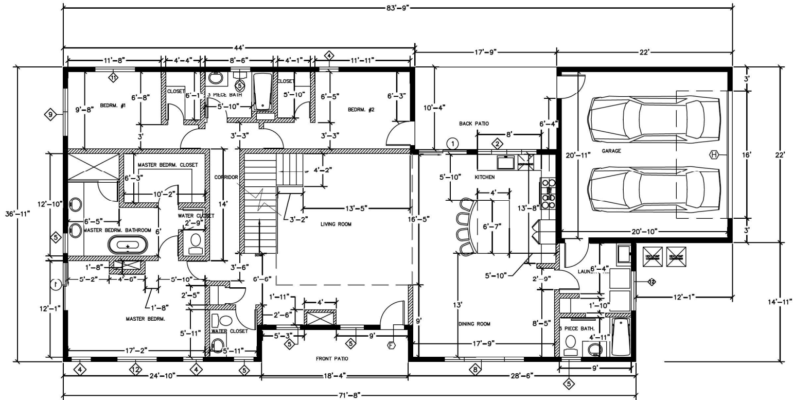
1 A1.1 MAIN FLOOR PLAN 1/8" = 1'-0" SCALE
